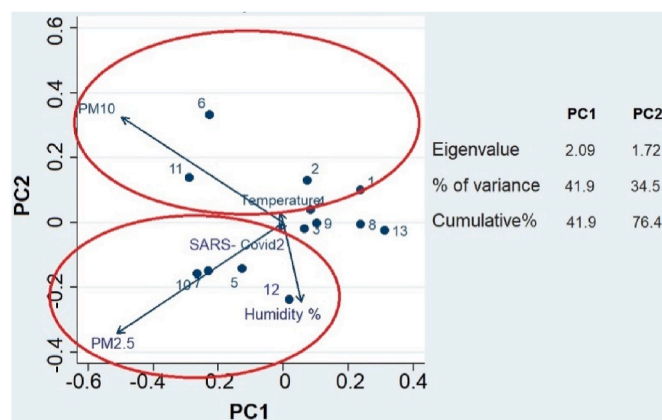
Fig. 3. Principal component analysis Biplot for the two principal components (PC1 vs PC2). SARS-CoV-2 is strongly correlated with humidity and PM 2.5 (lower red circle), but PM 10 and temperature are conversely correlated (upper red circle). Variable scores are plotted against the left and bottom axes.
